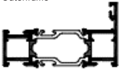
SPW700701 Outerframe
